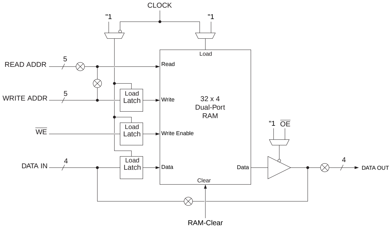
Figure 8. RAM Logic
